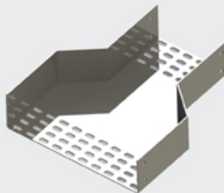
Central Reducer
